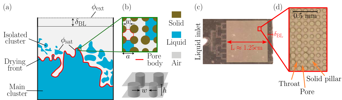
Figure 1. (a) Schematics of our model of isothermal drying of a horizontal porous sample open to the atmosphere at one of its faces. Low vapor concentration ( \phi = \phi_{\text{ext}} ) at the edge of a diffusive boundary layer (of thickness \delta_{\text{BL}} ) that develops outside the medium drives evaporation and vapor diffusion away from air-liquid interfaces (where \phi = \phi_{\text{sat}} ). Evaporation reduces liquid pressure, causing air to invade into liquid-filled pores. Some of the liquid disconnects from the bulk (i.e., the main cluster) and becomes isolated. The drying front, namely the leading part of the air-liquid interface (excluding isolated clusters), is marked in red. (b) We model evaporation, vapor diffusion and capillary invasion via a pore network model. Pores are defined as the space (delimited by a red line) between solid pillars (constant height h and variable radius R ) placed on a square lattice (spacing a ), and are interconnected by throats (aperture w ). (c) Drying experiments are performed in a horizontal microfluidic cell, initially filled with a volatile liquid via inlet channels. A boundary layer forms within an open region (pillar-free) of thickness \delta_{\text{BL}} . (d) Close-up image showing the solid cylindrical pillars (top view).
