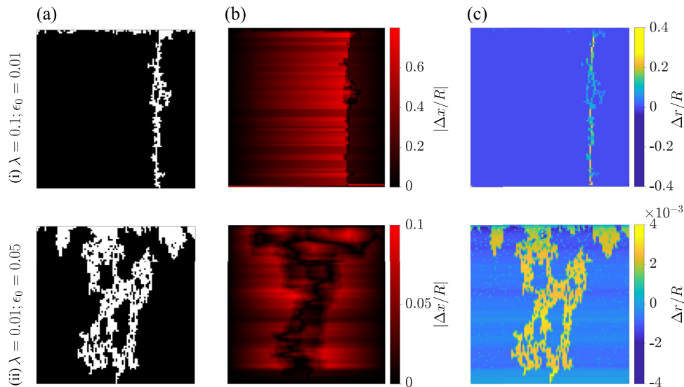
Fig. 7. Different mechanisms underlie deformation-assisted preferential drying when the deformation is induced by lowering confinement and lowering disorder: (i) Low initial confinement (top row, \epsilon_0 = 0.01 ) leads to large particle displacements and significant changes in throat apertures, while (ii) low disorder (bottom row, \lambda = 0.01 ) enhances the impact of small displacements. In both cases, the drying patterns at breakthrough are preferential (a). The magnitude of horizontal particle displacement |\Delta x/R| is significantly larger for low \epsilon_0 than for low \lambda , and centered around the invading air finger (b). Consequently, changes in vertical throat apertures \Delta r/R are more pronounced for low \epsilon_0 (c). We note that at low disorder, even small aperture changes impact the drying pattern, as evident from the equivalence of the pattern and deformations (panels a and c in bottom row). This is highlighted by the different scale in which the deformations are presented (panels b and c).
