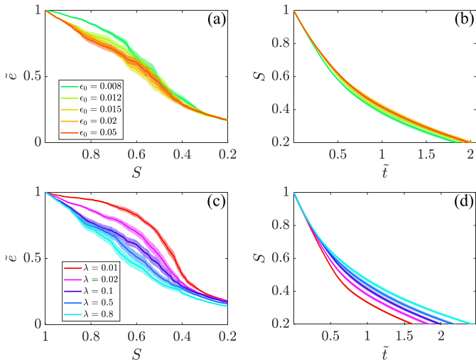
Fig. 6. Drying curves (rate vs. saturation), and the temporal evolution of the saturation. The drying rate \bar{e} decreases more gradually for lower \epsilon_0 values (a), mostly in the initial stages of drying, with a relatively limited effect on \tilde{t} (b). Similarly, \bar{e} decreases more gradually for lower \lambda (c), resulting in shorter drying time \tilde{t} (d). Solid lines and shaded area represent the mean value and standard error, respectively, calculated from 20 realizations for each \lambda or \epsilon_0 value. We use a fixed value of \lambda = 0.1 for the simulations in a–b, and \epsilon_0 = 0.05 for c–d.
