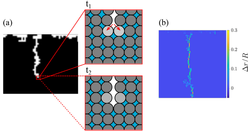
Fig. 3. Preferential drying is associated with matrix deformation. The air finger in panel (a) is the consequence of progressive pore opening due to pressure imbalance (capillary pressure) acting on the particles at the finger tip. The insets show the particle positions (gray circles), before ( t_1 ) and after ( t_2 ) a particular pore invasion event, featuring the enlargement of the throat formed between the particle pair (highlighted in light gray) at the finger tip due to the pressure imbalance pushing the particles apart. Red arrows indicate the resultant pressure force acting on the particles, increasing the throat aperture and facilitating the next pore invasion at the finger tip, unless a larger throat is already accessible elsewhere. Air and liquid filled pores appear in white and blue, respectively. Panel (b) shows the change in the throat apertures, \Delta r , rescaled by the particle radius R (for simplicity only the vertical throats are plotted). If this deformation-assisted mechanism is dominant, the macroscopic drying pattern follow the path of the modified throat apertures, making it highly preferential, leaving most of the liquid behind at breakthrough. (For interpretation of the references to colour in this figure legend, the reader is referred to the web version of this article.)
