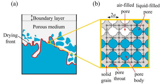
Fig. 1. (a) Model schematics. The porous medium is open at one of its faces, where a vapor concentration gradient drives evaporation from the air-liquid interface, and out to the atmosphere through a diffusive boundary layer. As evaporation reduces liquid pressure, air invades into liquid-filled pores. Some of the liquid becomes disconnected and forms isolated clusters. The drying front (in red) represents the most advancing part of the interface. (b) We model evaporation and capillary invasion via a pore network model, which we couple with a block-spring model that captures the effect of capillary pressures on matrix deformation. Pore bodies represent the space between solid particles placed on a square lattice (with spacing of 2a ), and are interconnected by throats. Solid particles are illustrated here as dented blocks, a 2-D illustration that emphasizes that our model considers a network of contact forces between particles (represented by springs), while allowing fluid connectivity between the pores. Displacement of solid particles modifies the pore throats, impacting their capillary thresholds. (For interpretation of the references to colour in this figure legend, the reader is referred to the web version of this article.)
